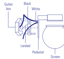
ELECTRIC DIAGRAM (W) White wire: Neutral (B) Black wire: Line (⊕) Copper wire: Ground
